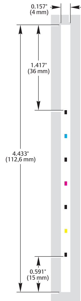
Autotron 4-Color Circumferential Marks
