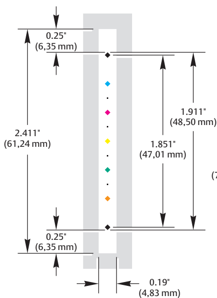
6-color Circumferential Marks
